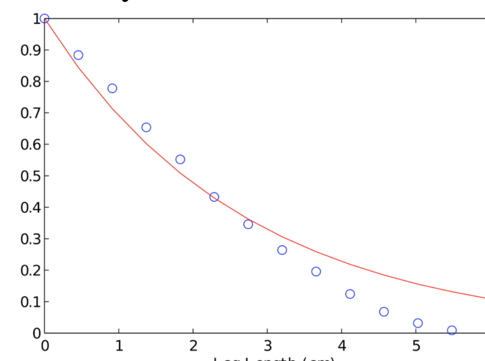
Figure. 2 A plot of the auto-correlation from a magnetic probe signal
