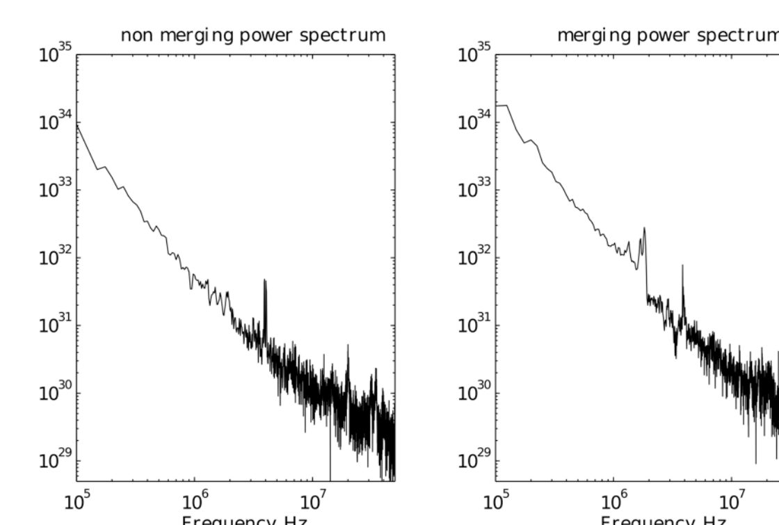
Figure. 11 Merging and non-merging power spectrum comparison from the He-Ne interferometer showing a feature around 2 MHz during merging
