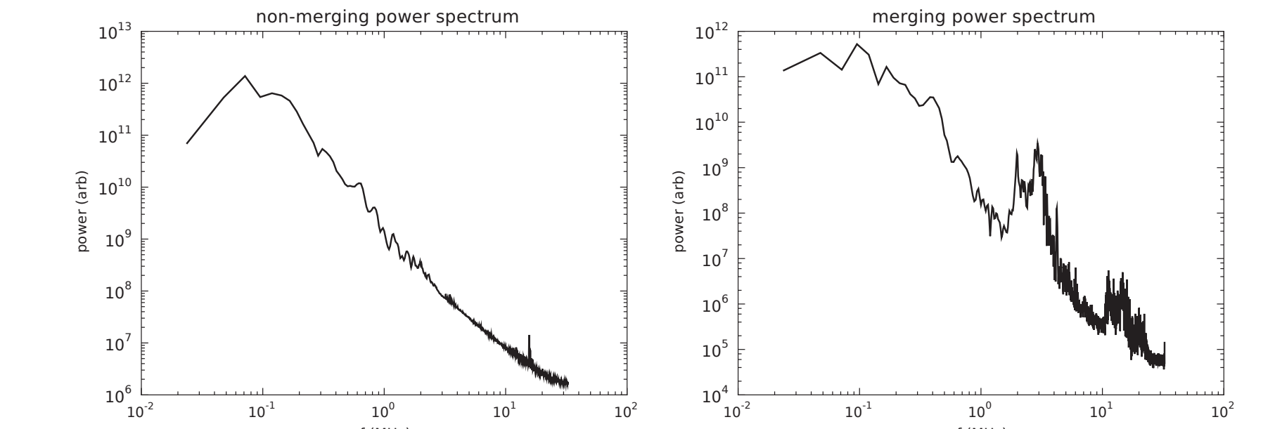
Figure. 12 Power spectra from the radial magnetic probe showing the same 2 MHz feature present only in the merging case
