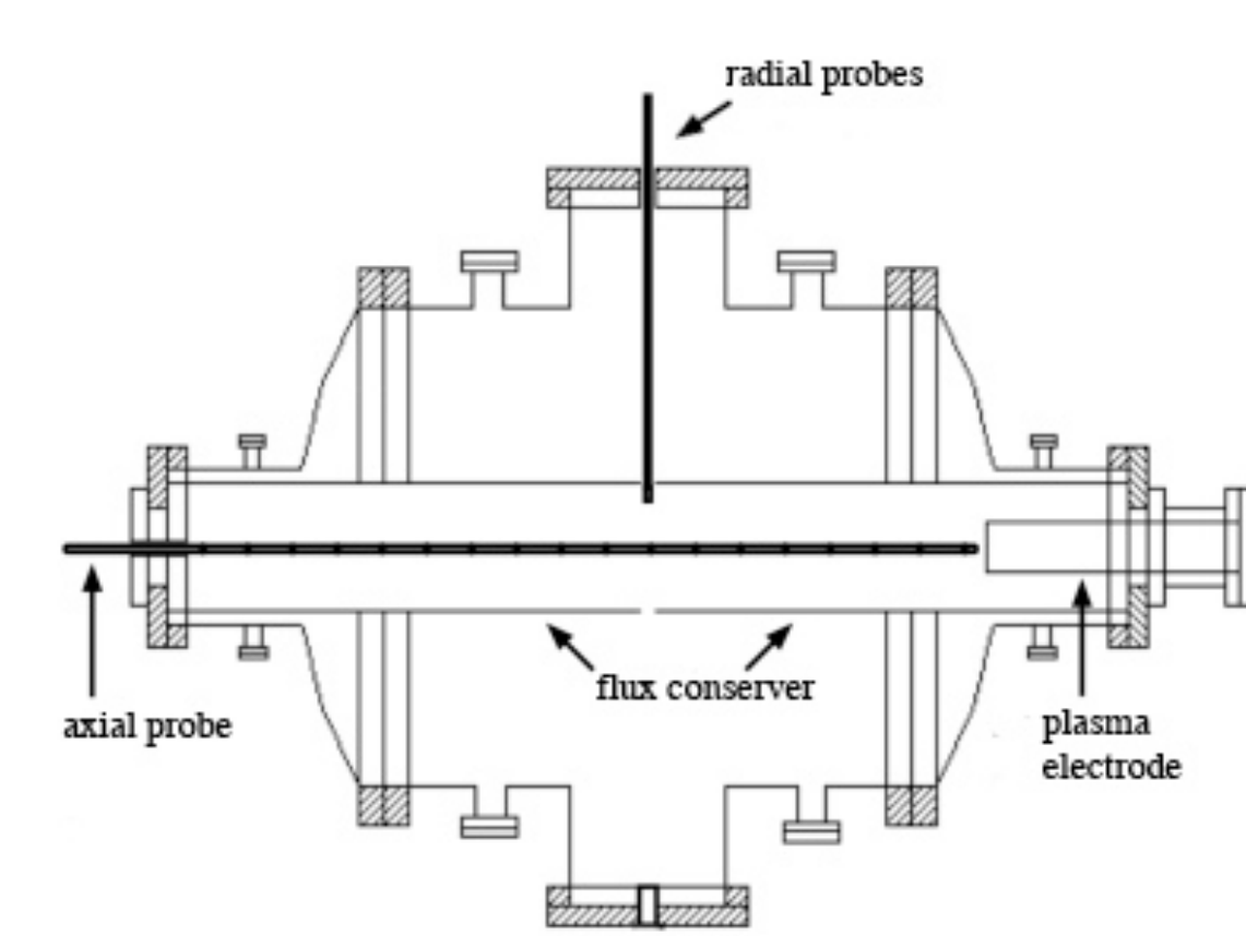
Figure. 4 SSX setup showing the magnetic probes
