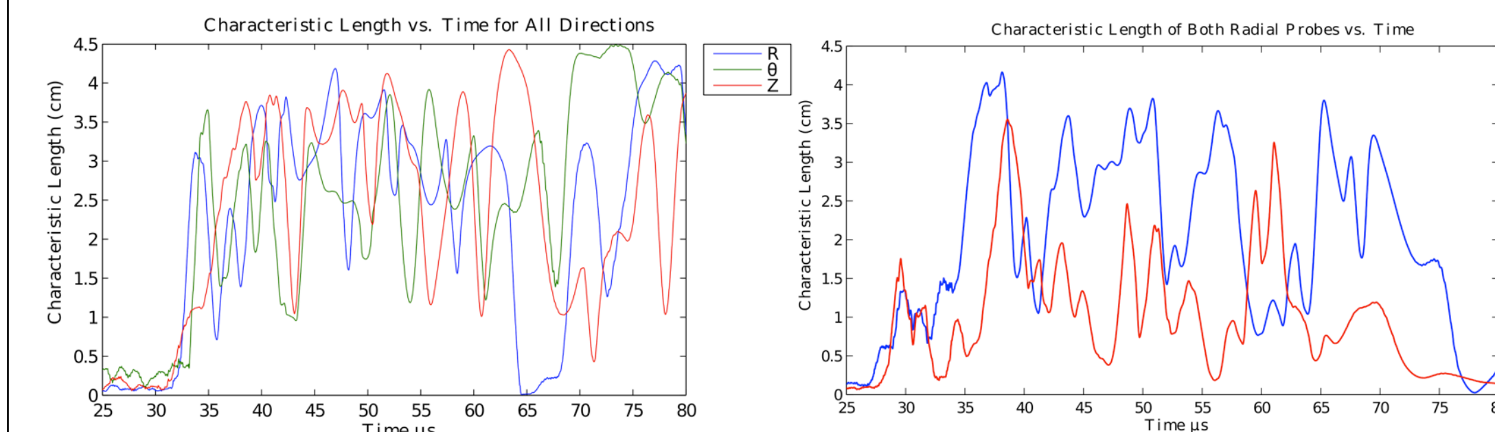
Figure. 9,10 Comparison of the characteristic length (Eq. 3) in time from both radial probes showing the shift from being similar early in time to being nearly opposite later (right) and a comparison of the three directions from a single probe (left)
