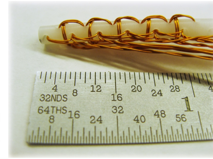
Figure. 3 One of the radial probes during construction
