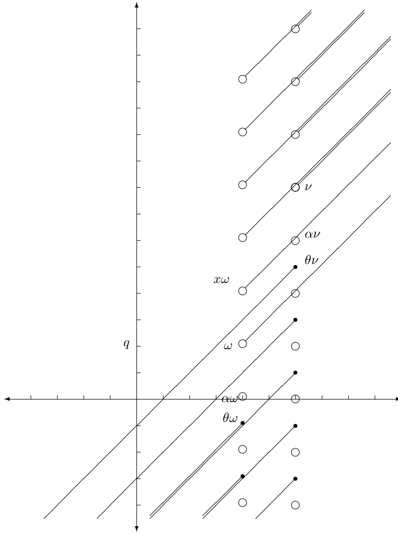
FIGURE 7. d(\omega) = \theta\nu/x^\ell y^k
